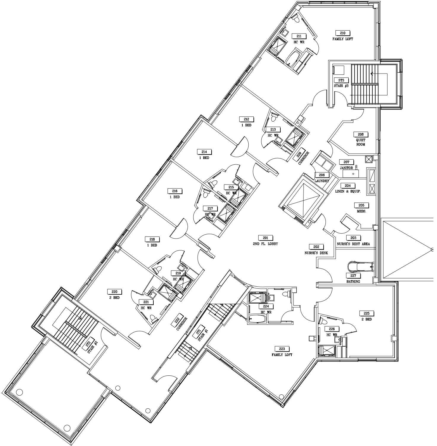
2 A900 ROGER'S HOUSE SECOND FLOOR SCALE 1:100
